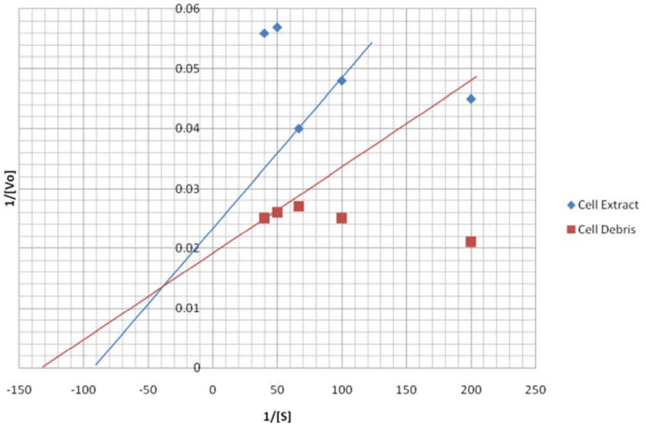
Figure 5. Lineweaver-Burk plots of NDMA formation in cell extract and cell debris of Bacillus cereus at a fixed DMA concentration and varying NaNO 2 concentrations.
