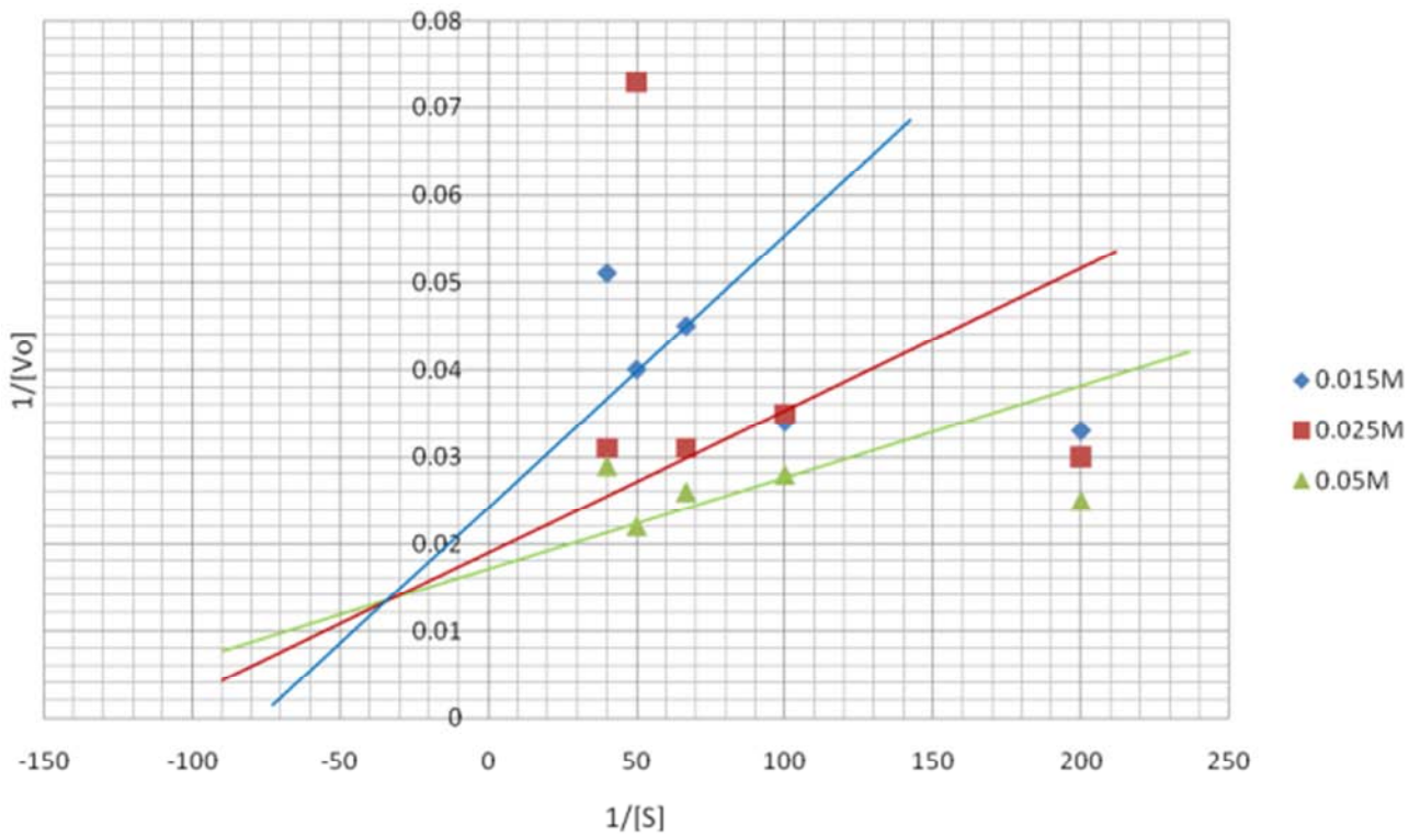
Figure 6. Lineweaver-Burk plots of nitrosation by cell debris of Bacillus cereus incubated with a fixed concentration of dimethylamine at different concentrations of sodium nitrite.
