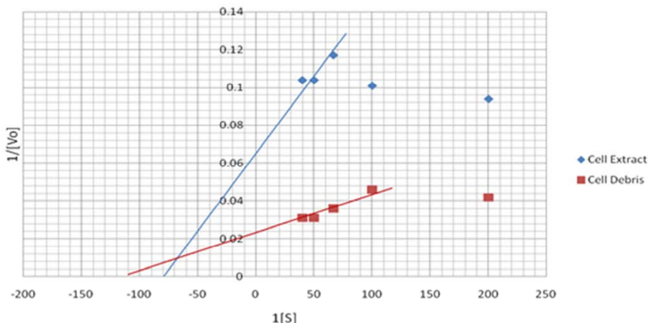
Figure 4. Lineweaver-Burk plots of NDMA formation in cell extract and cell debris of Bacillus cereus at a fixed \text{NaNO}_2 concentration and varying DMA concentrations.
